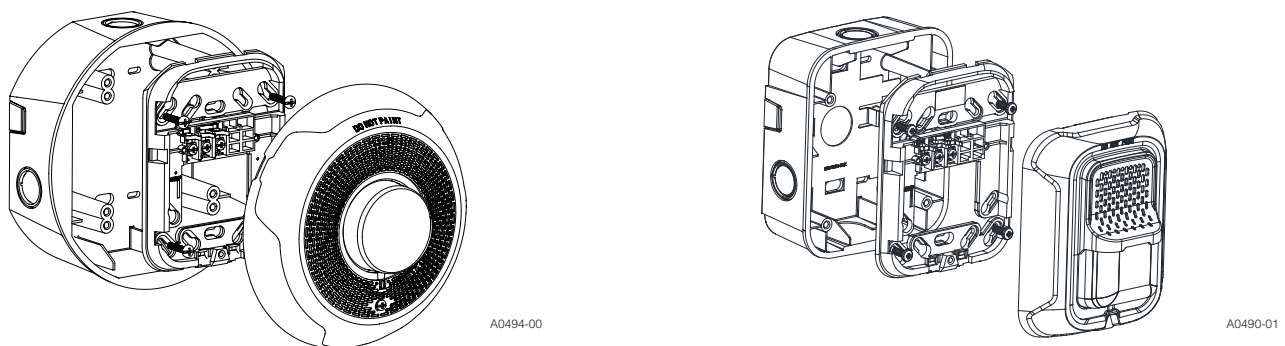
Ceiling Mount Chime/Strobe with Ceiling Surface Mount Back Box
