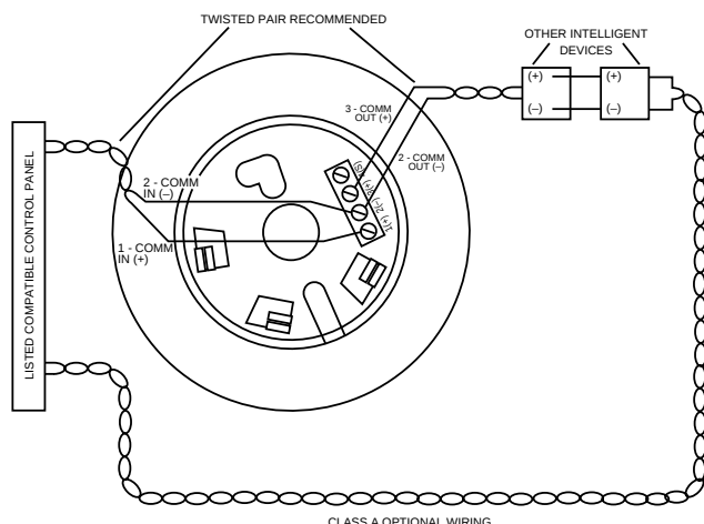
Isolator Base
