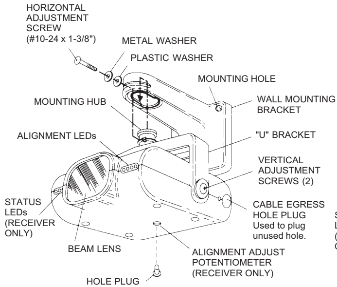
▲ Wall Mounting
