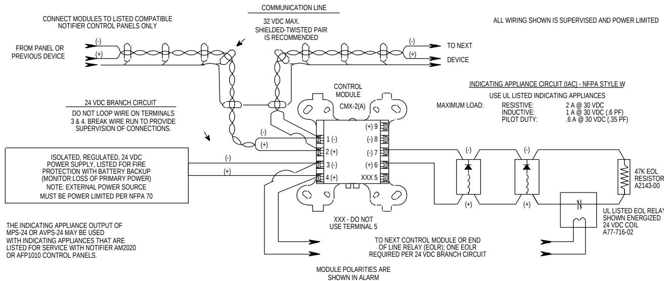
FIGURE 5. TYPICAL INDICATING CIRCUIT CONFIGURATION, NFPA STYLE W
