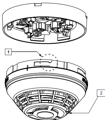
Figure 1: KI-OSHD features
