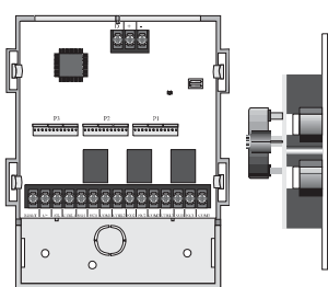
FC-2880 Annunciator Driver Module
