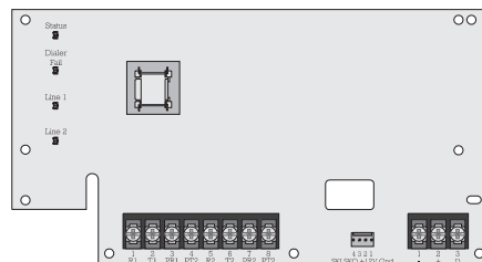
FC-2104 Digital Alarm Communicator Transmitter
