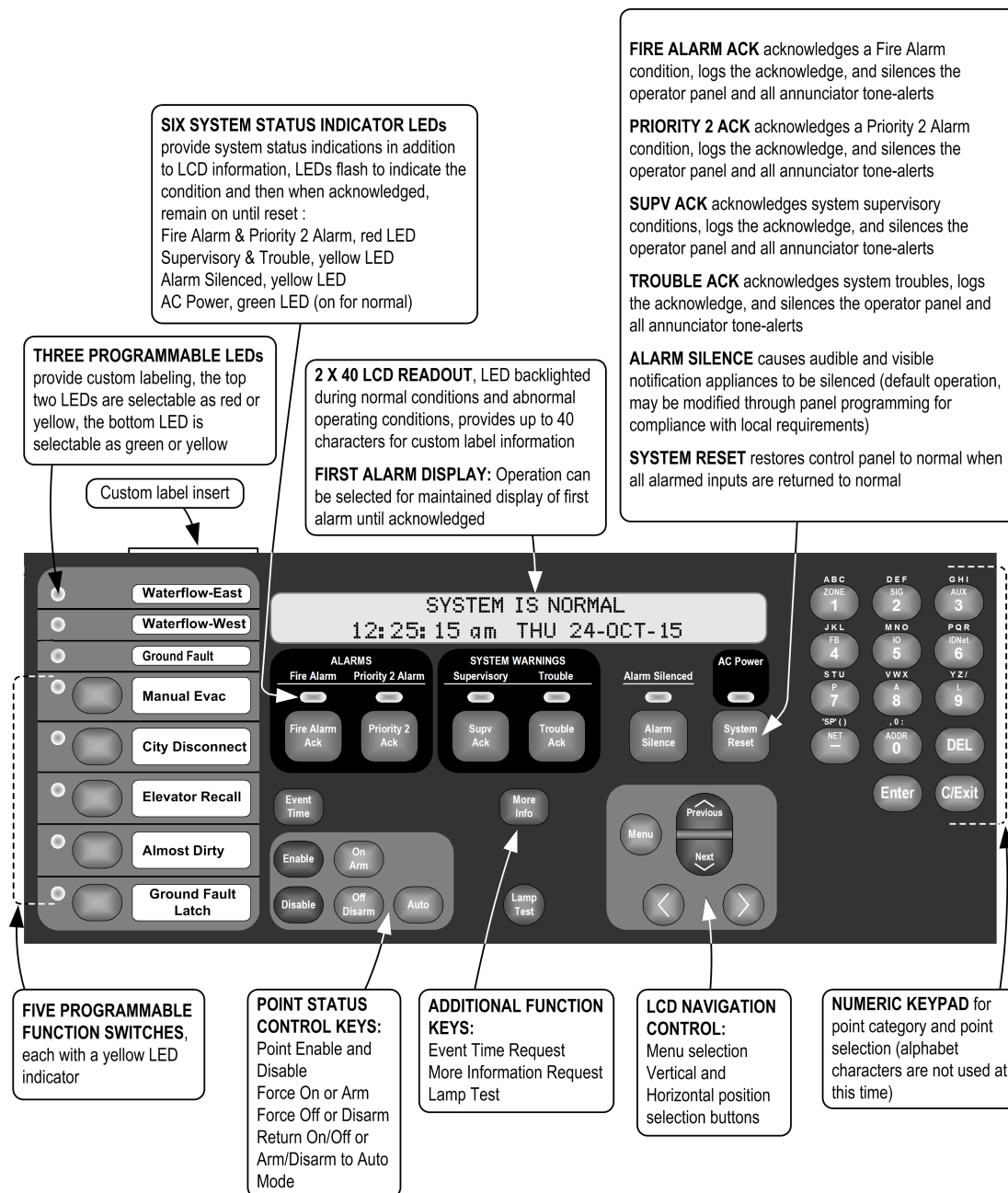
Figure 16: Operator interface
