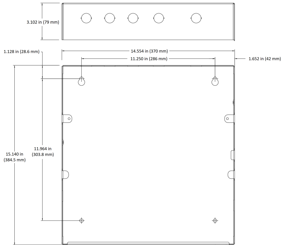
Figure 4: Cabinet details
